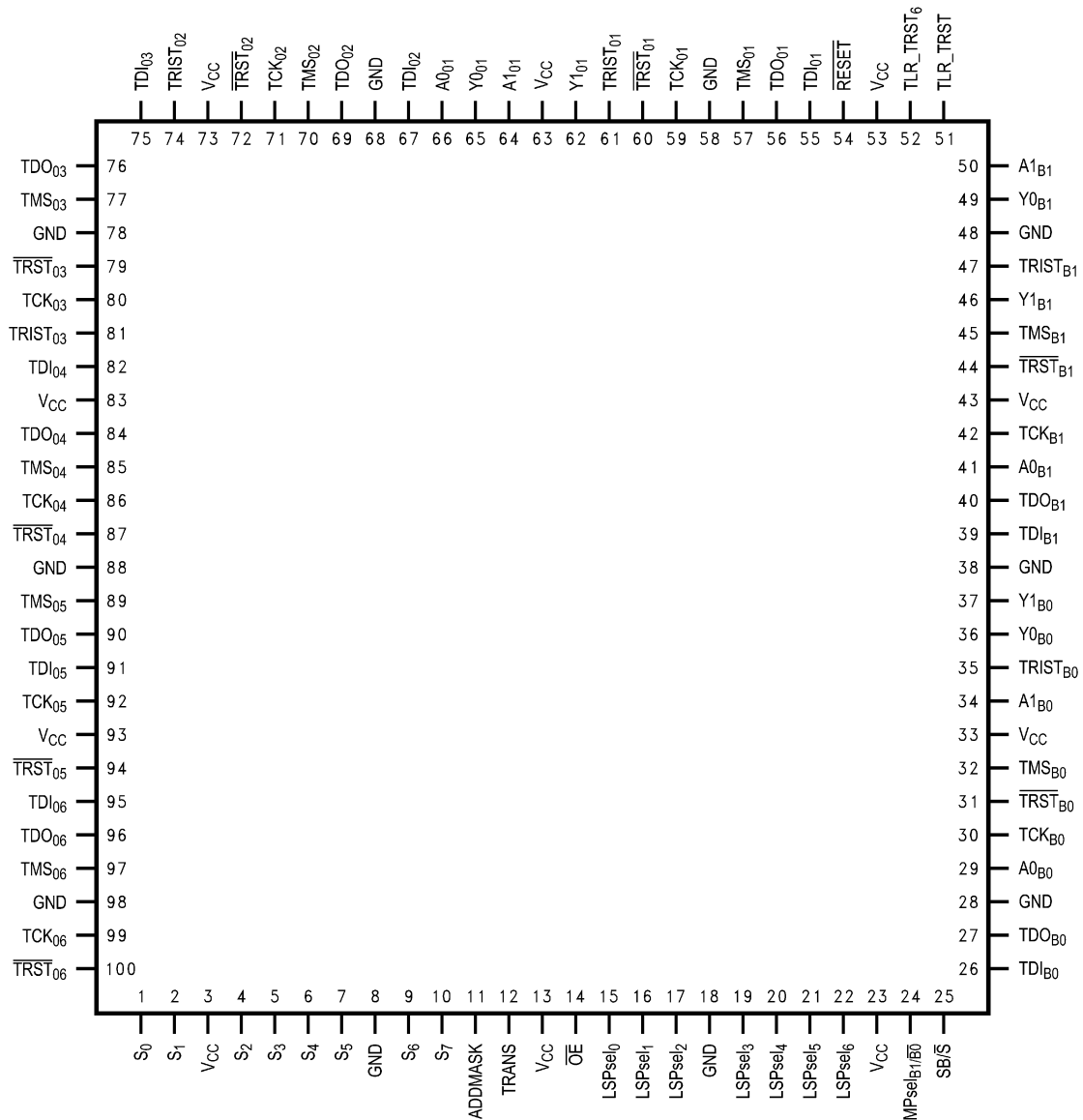
Figure 5. TQFP pinout
