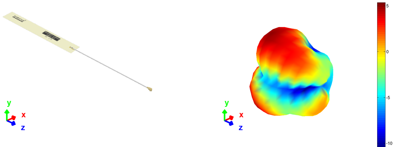
3D pattern at 657MHz
