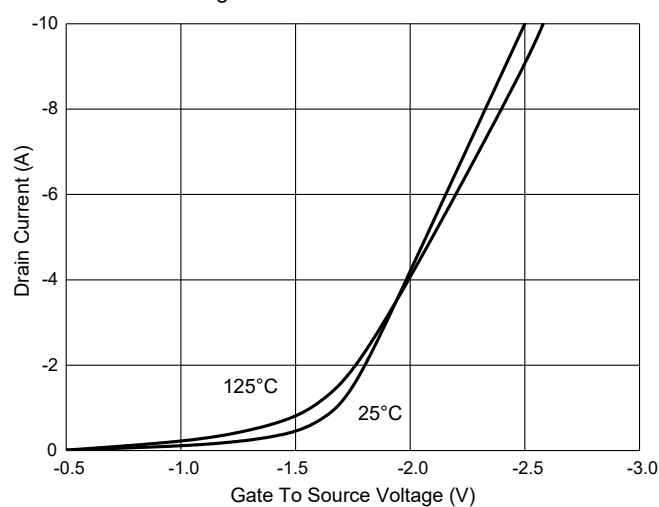
Fig. 9 - Transfer Characteristics
