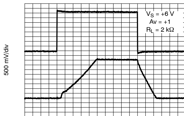
Figure 29. 6 V Non-Inverting Large Signal Pulse Response
