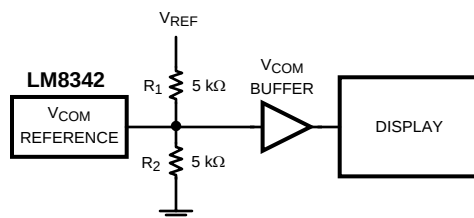
Figure 40. VCOM Buffer
