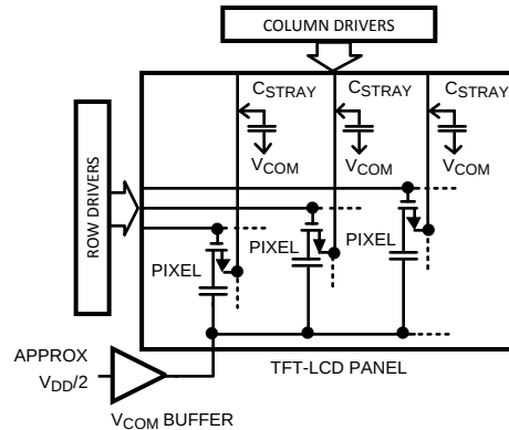
Figure 31. TFT Display
