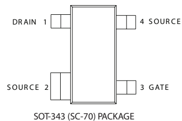
SOT-343 (SC-70) PACKAGE
