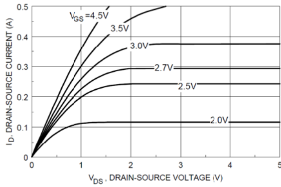
Figure 1. On-Region Characteristics
