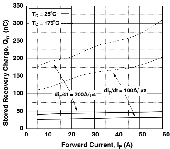
Figure 23. Stored Charge
