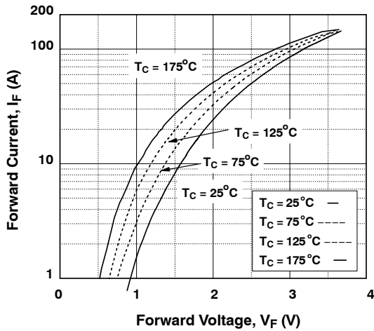
Figure 21. Forward Characteristics
