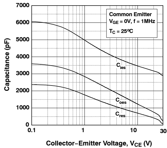
Figure 9. Capacitance Characteristics
