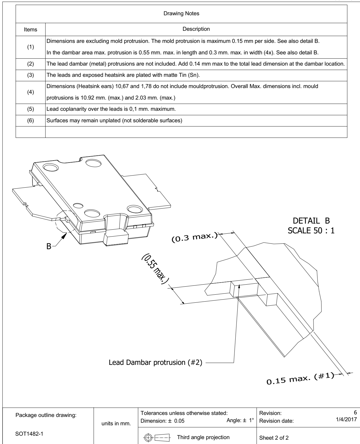
Fig 19. Package outline SOT1482-1 (sheet 2 of 2)
