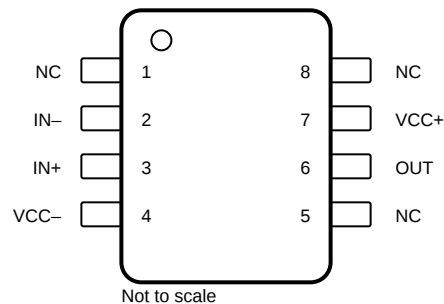
Figure 5-2. TL081H D Package 8-Pin SOIC Top View
