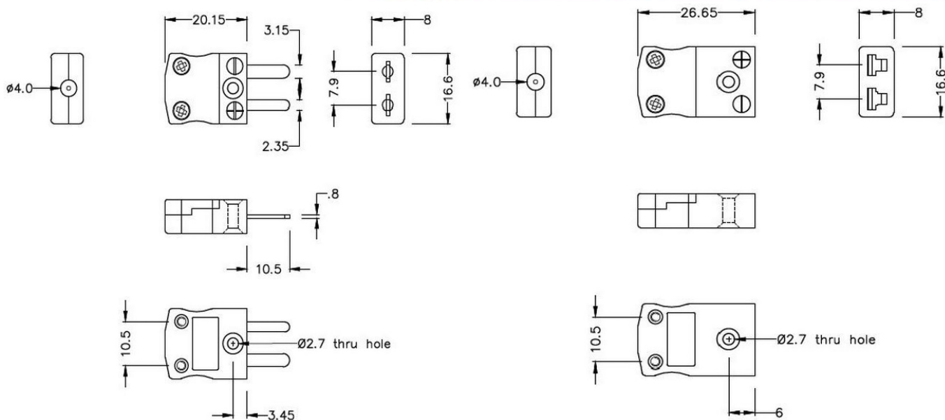
Miniature in-line Socket (dimensions in mm)
