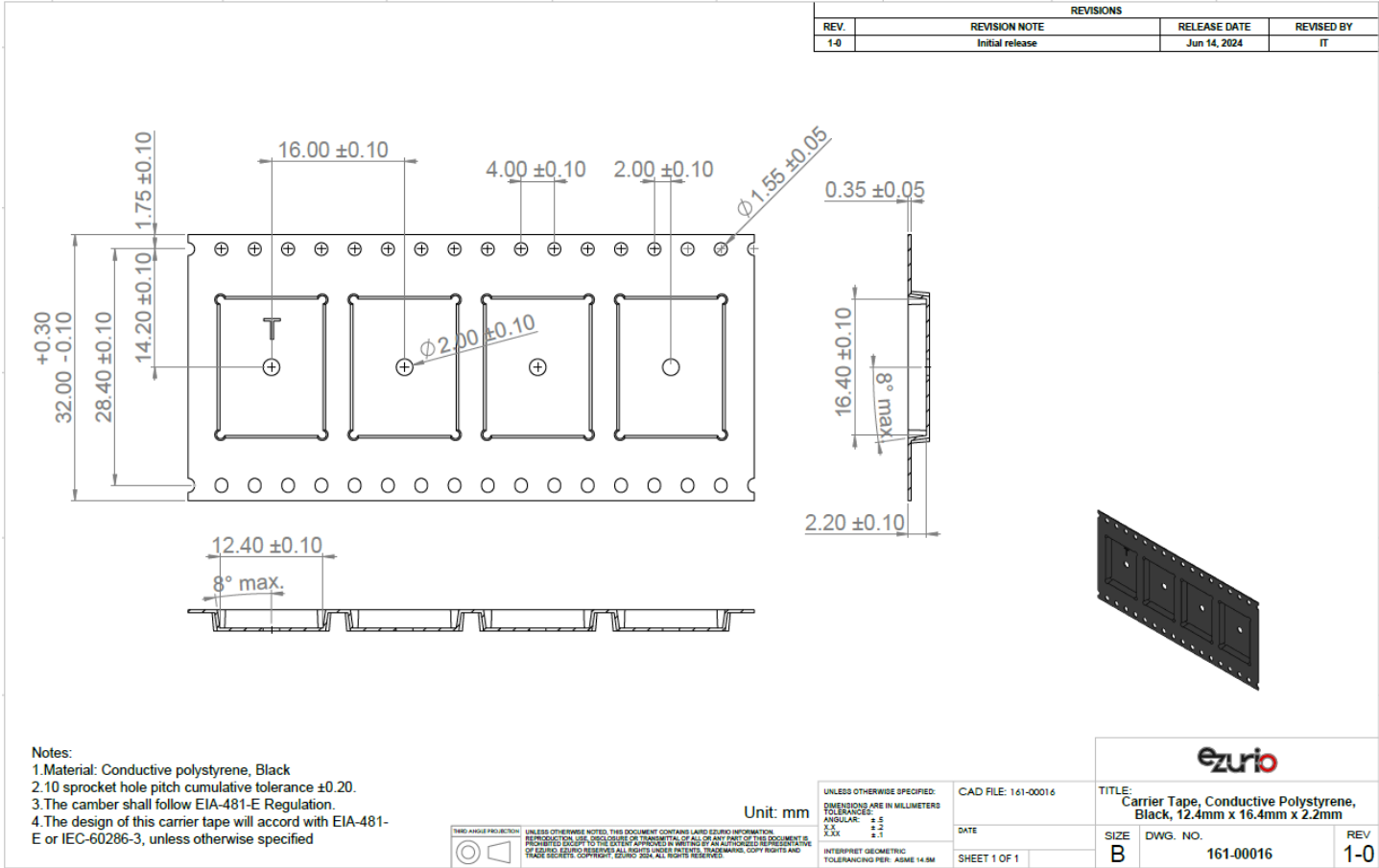
Figure 24: Sona IF513 Tape specifications, 161-00016
