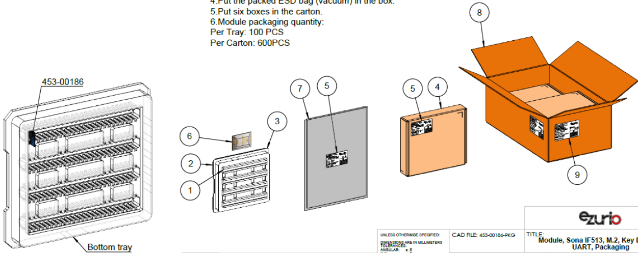
Figure 31: Sona IF513 M.2 2230 Packaging Process, 453-00186-PKG
