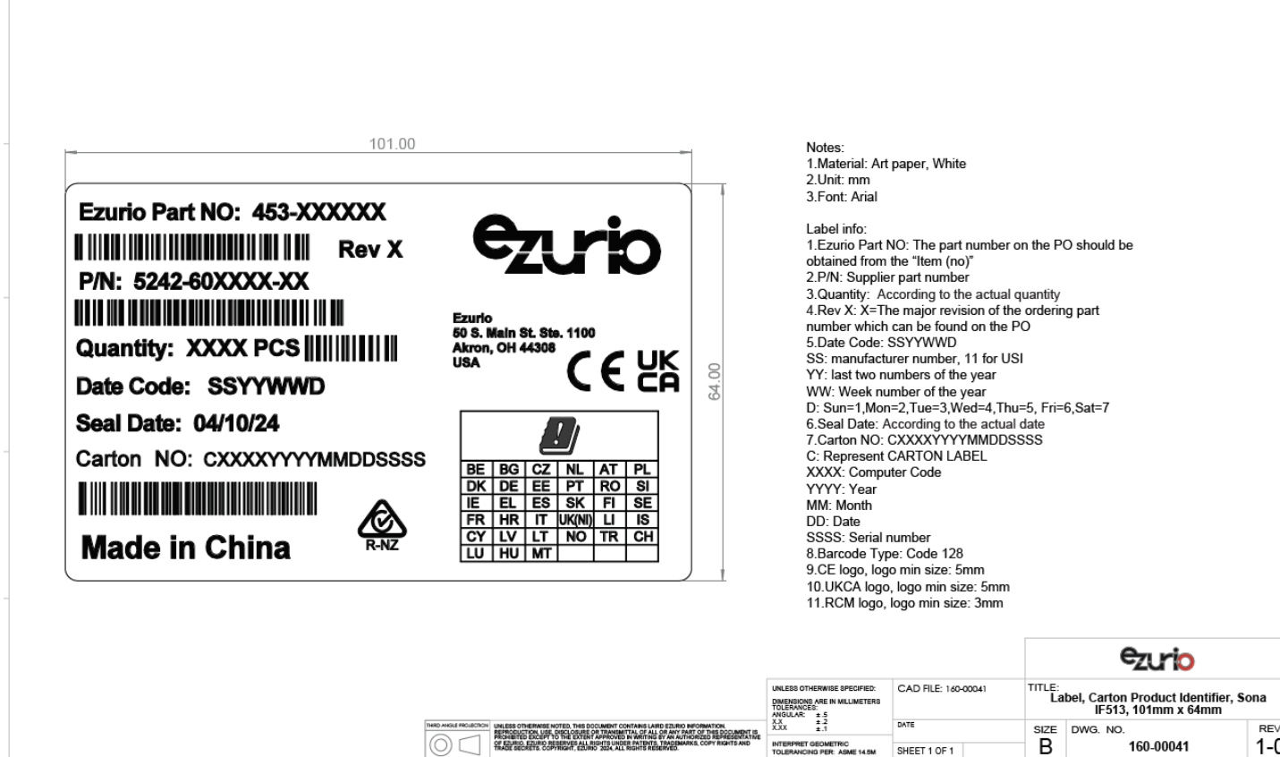
Figure 28: Sona IF513 Carton Product Identifier Label, 160-00041
