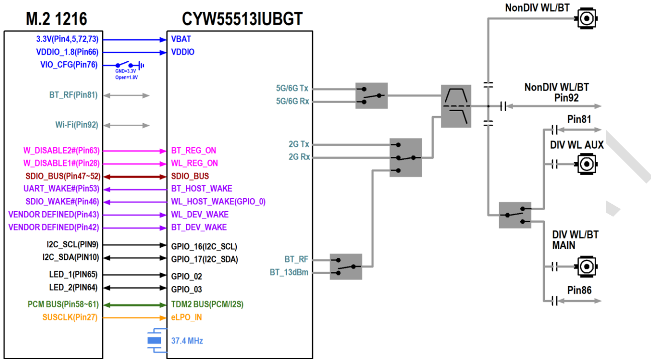
Figure 1: M.2 1216 Solder-Down type block diagram
