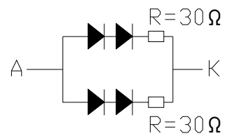
Curcuit Diagram
