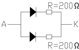
Curcuit Diagram
