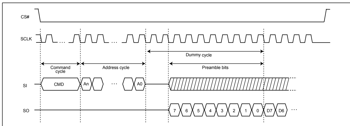
Figure 44. SDR 1I/O (10DC)
