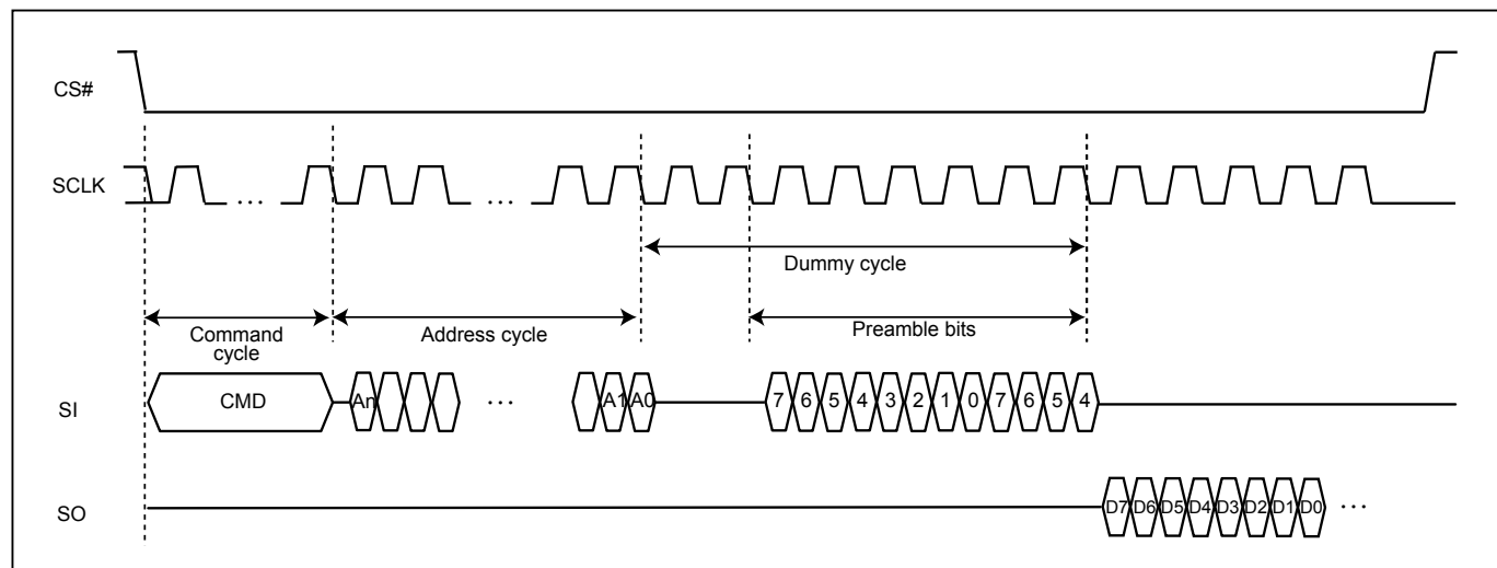
Figure 50. DTR1IO (8DC)
