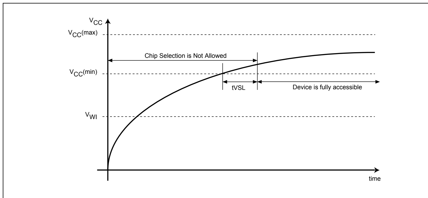
Figure 121. Power-up Timing
