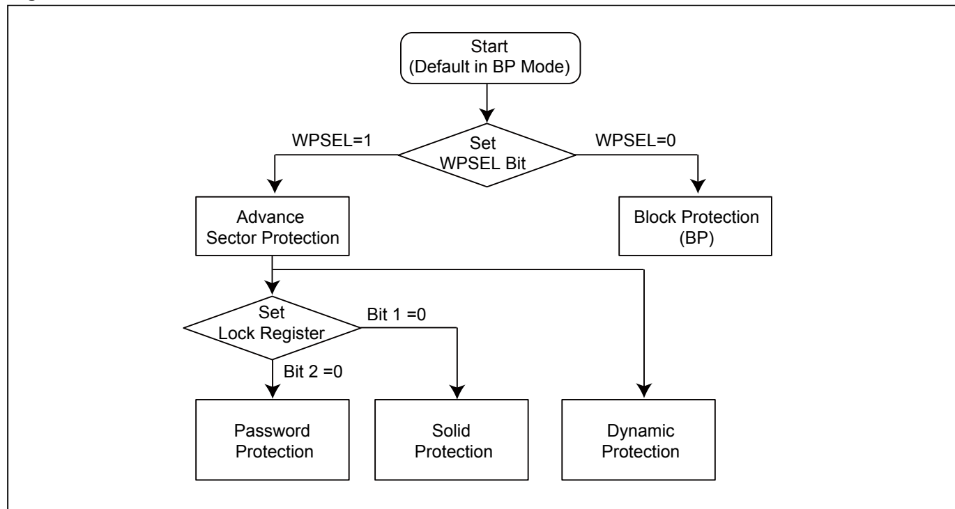
Figure 91. Write Protection Selection
