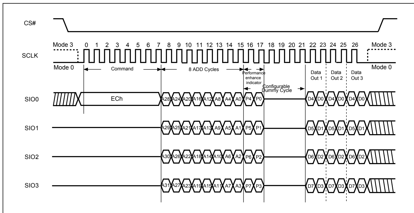
Figure 57. 4 I/O Fast Read using 4 Byte Address sequence (4READ4B)
