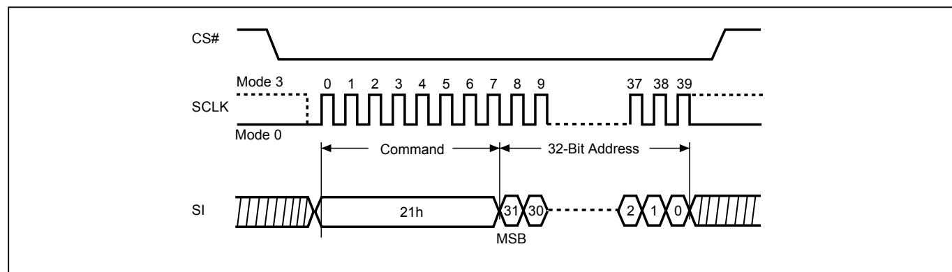
Figure 62. Sector Erase (SE4B) Sequence (SPI Mode)
