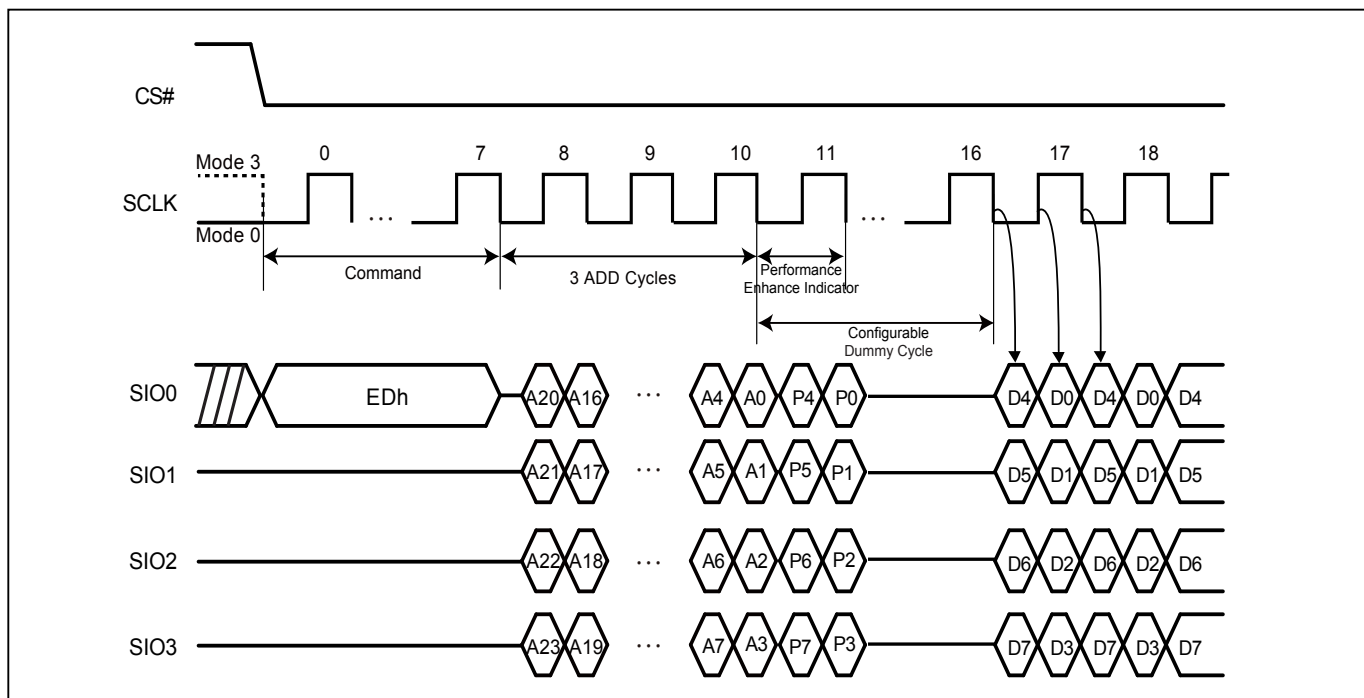
Figure 42. Fast Quad I/O DT Read (4DTRD) Sequence (SPI Mode)
