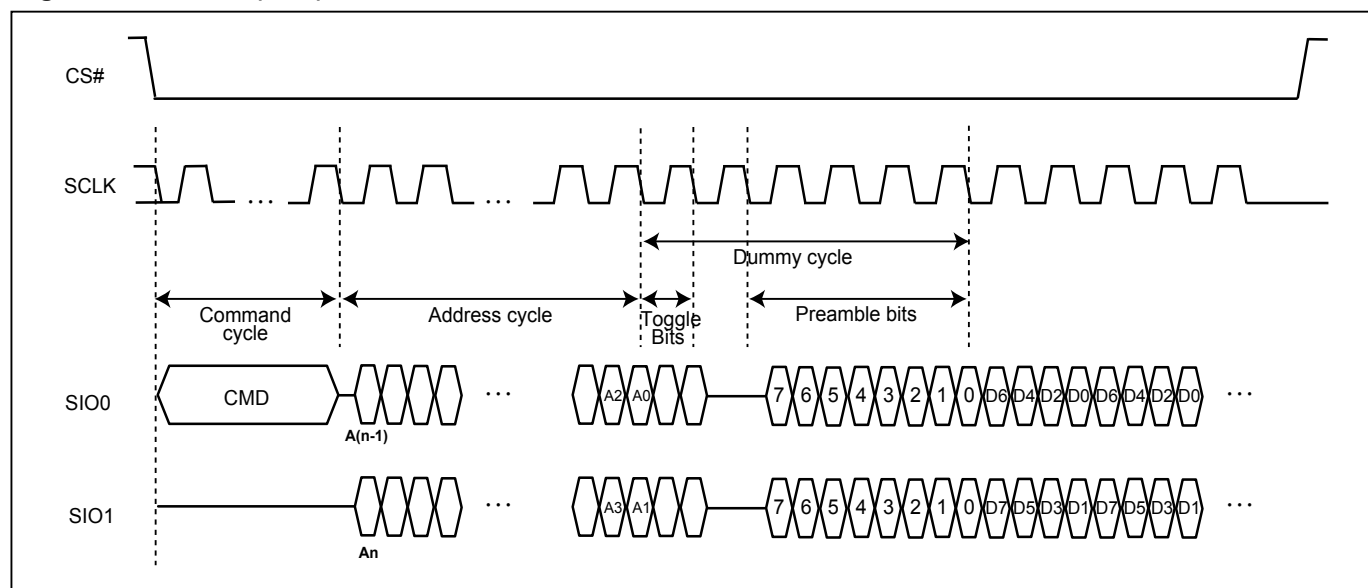
Figure 51. DTR2IO (6DC)
