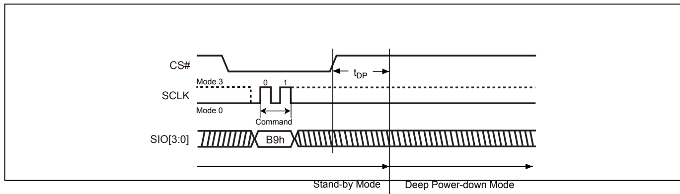
Figure 90. Deep Power-down (DP) Sequence (QPI Mode)
