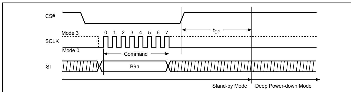
Figure 89. Deep Power-down (DP) Sequence (SPI Mode)
