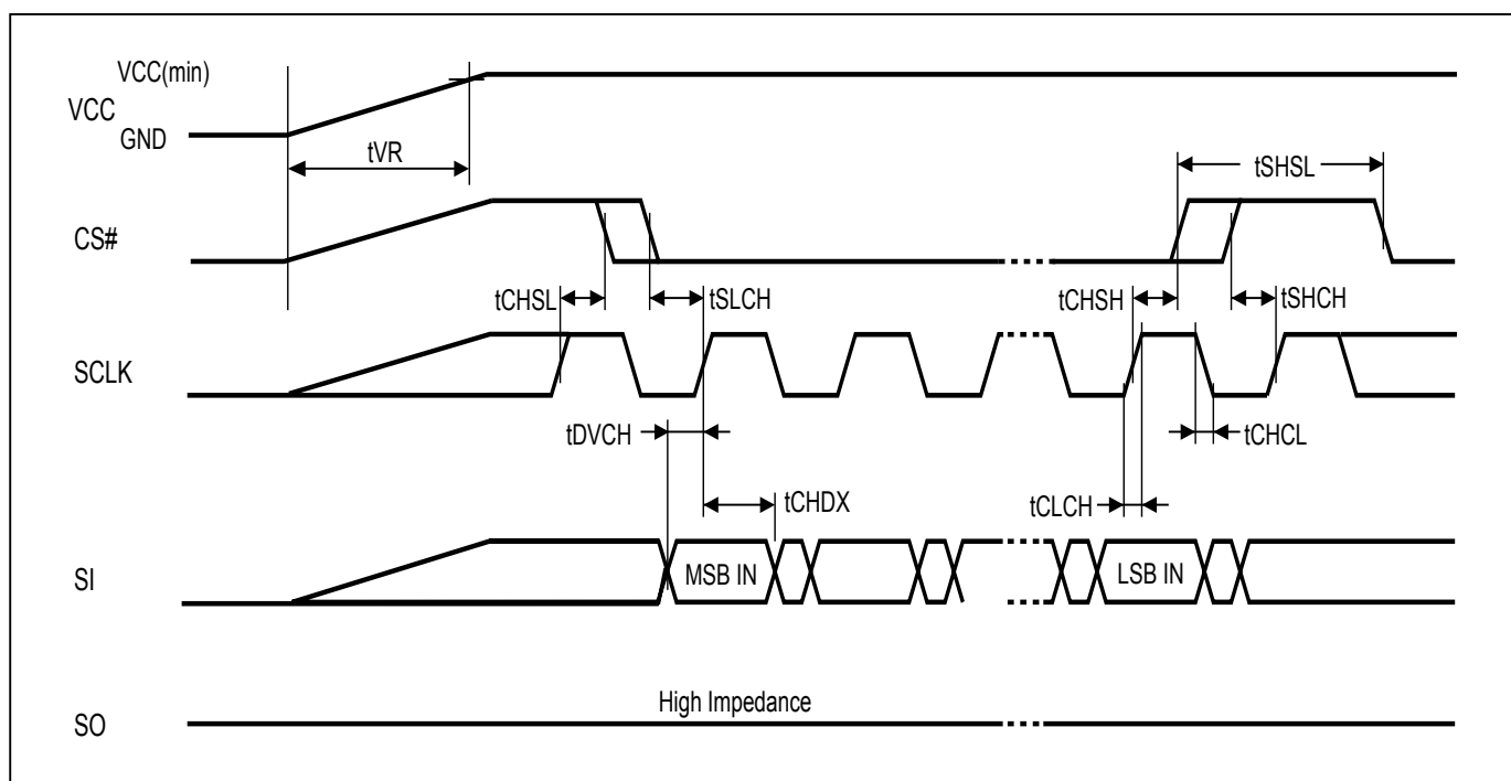
Figure 119. AC Timing at Device Power-Up
