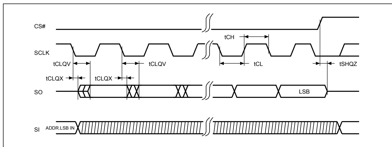
Figure 3. Output Timing (STR mode)
