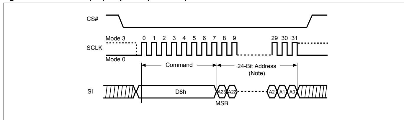
Figure 82. Block Erase (BE) Sequence (SPI Mode)
