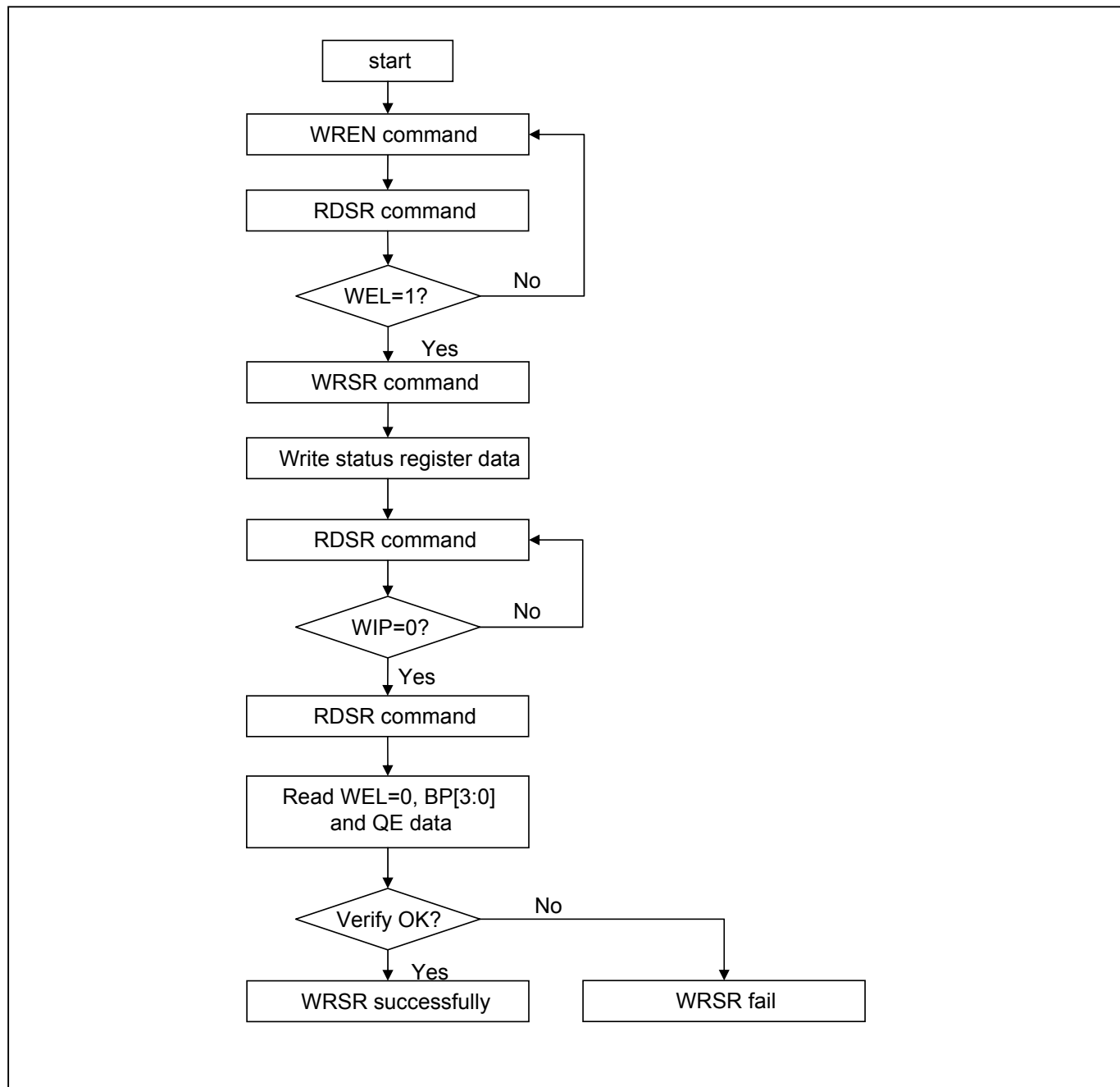
Figure 32. WRSR flow
