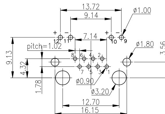
PCB Layout Component Side Shown
