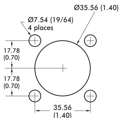
REAR MOUNT OPTION A **
