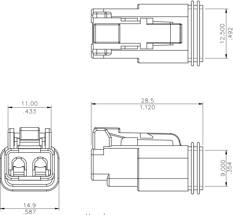
Housing
