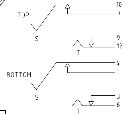
SCHEMATIC
