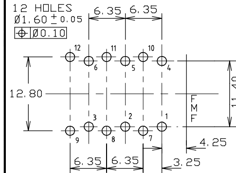
PC LAYOUT (COMPONENT SIDE)
