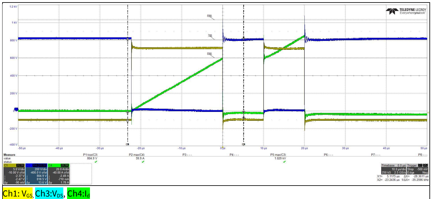
Figure 4 Eval-1ED3145MC12H-SiC – Double-pulse test of the low-side CoolSiC™ MOSFET
