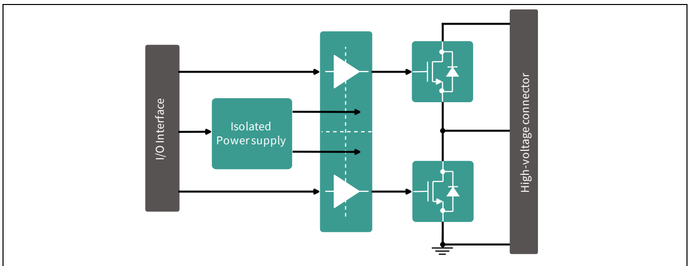
Figure 2 Eval-1ED3145MC12H-SiC evaluation board block diagram
