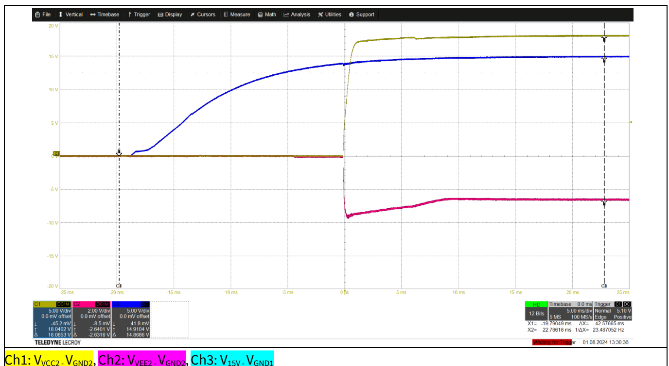
Figure 3 Eval-1ED3145MC12H-SiC – Power supply voltages startup
