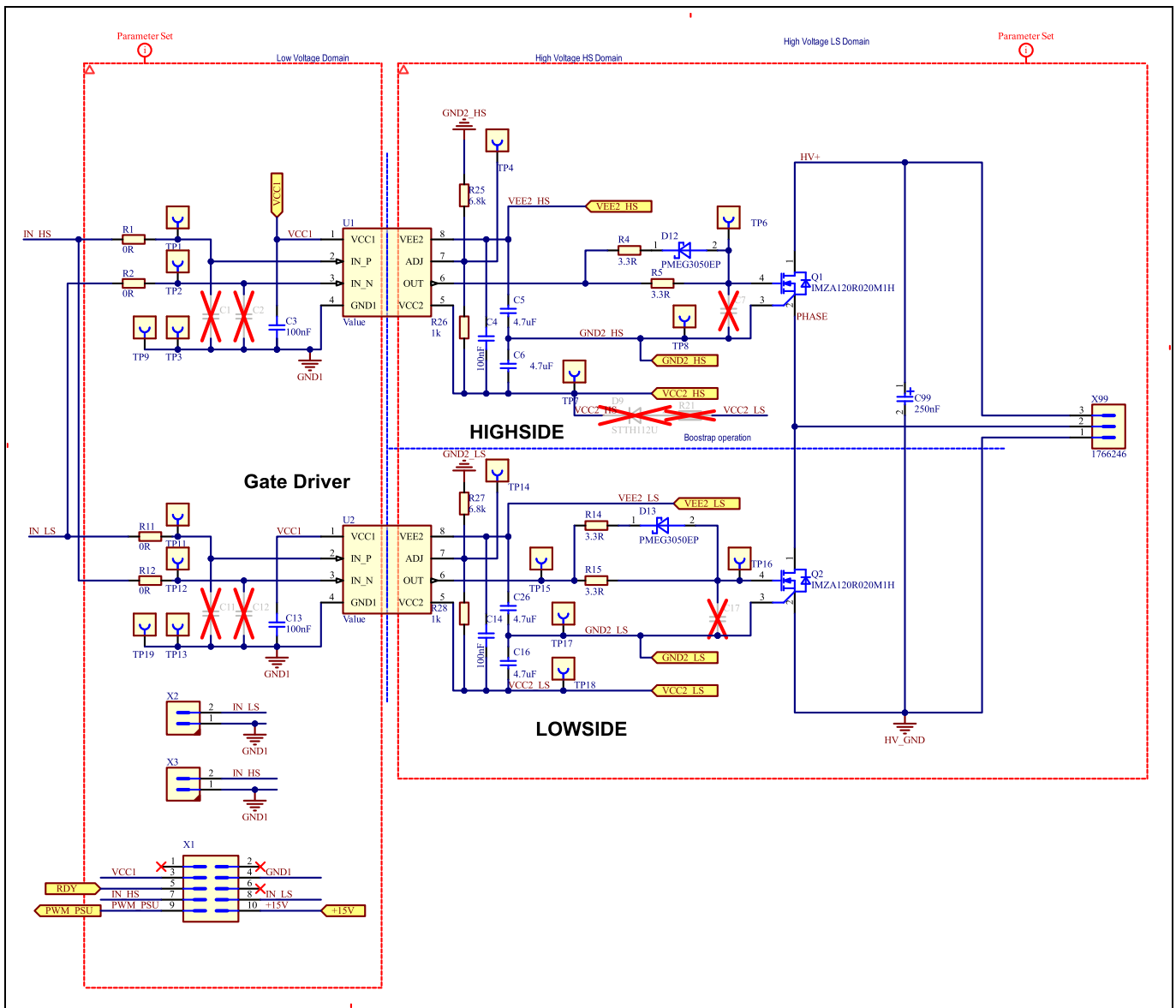
Figure 8 Gate driver circuit schematic
