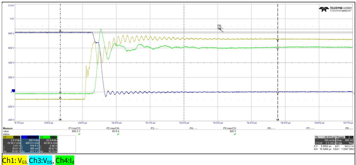
Figure 5 Eval-1ED3145MC12H-SiC – Turn-on of the low-side CoolSiC™ MOSFET
