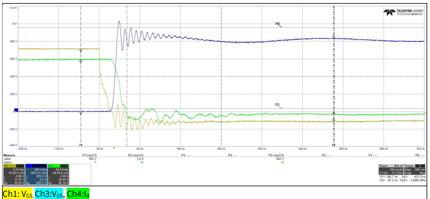
Figure 6 Eval-1ED3145MC12H-SiC – Turn-off of the low-side CoolSiC™ MOSFET
