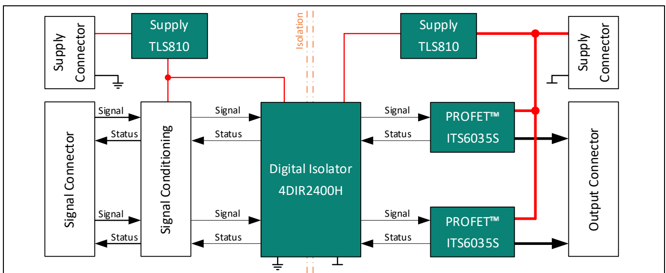
Figure 1 Block diagram
