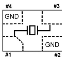
Top view connections (#2 & #4: connected to metal lid)
