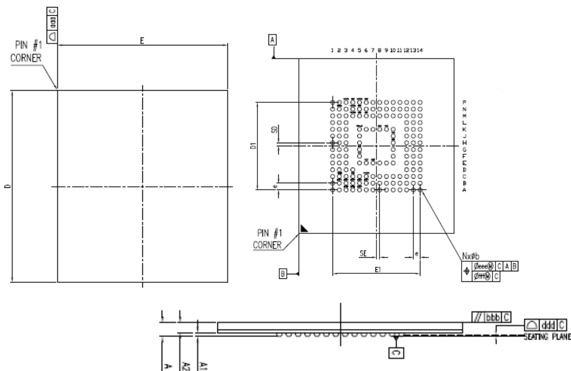
Figure 2 – Package Dimensions
