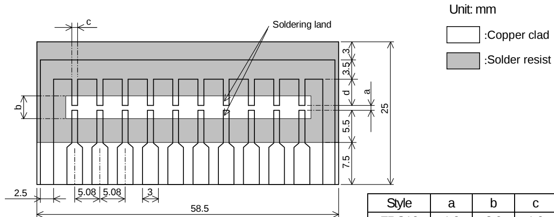
FRC16, 20 TEST SUBSTRATE
