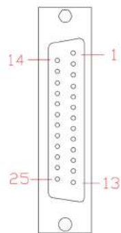
DB25 M
