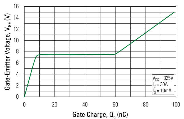
Fig. 8. Gate Charge
