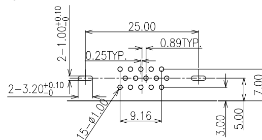
RECOMMENDED PCB LAYOUT TOLERANCE: \pm 0.05 mm
