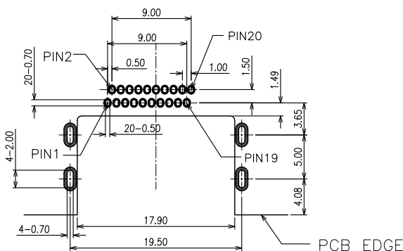
RECOMMENDED PCB LAYOUT TOLERANCE: ±0.05mm
