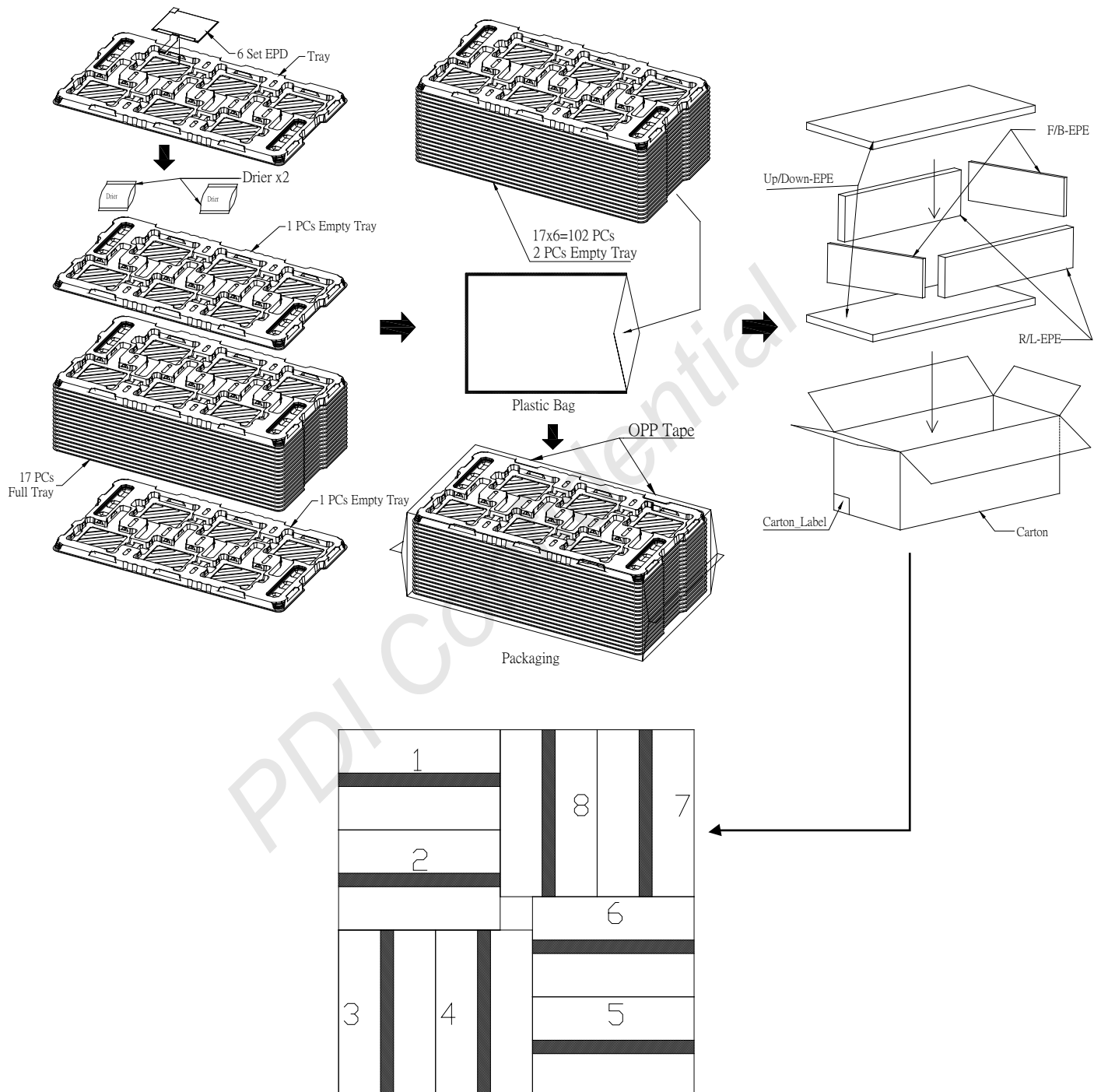
Figure 7-1 Packing Diagram
