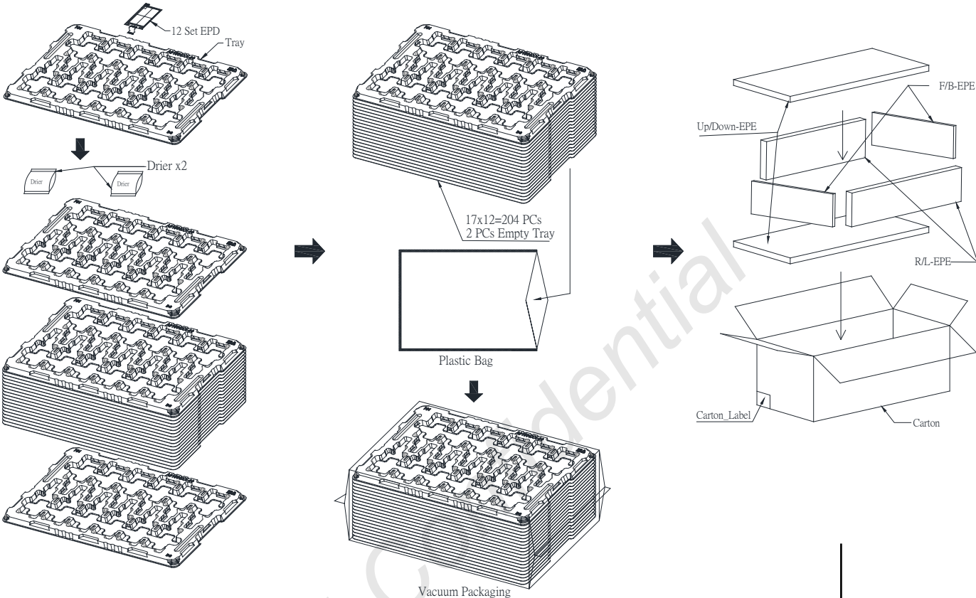
Figure 7-1 Packing Diagram
