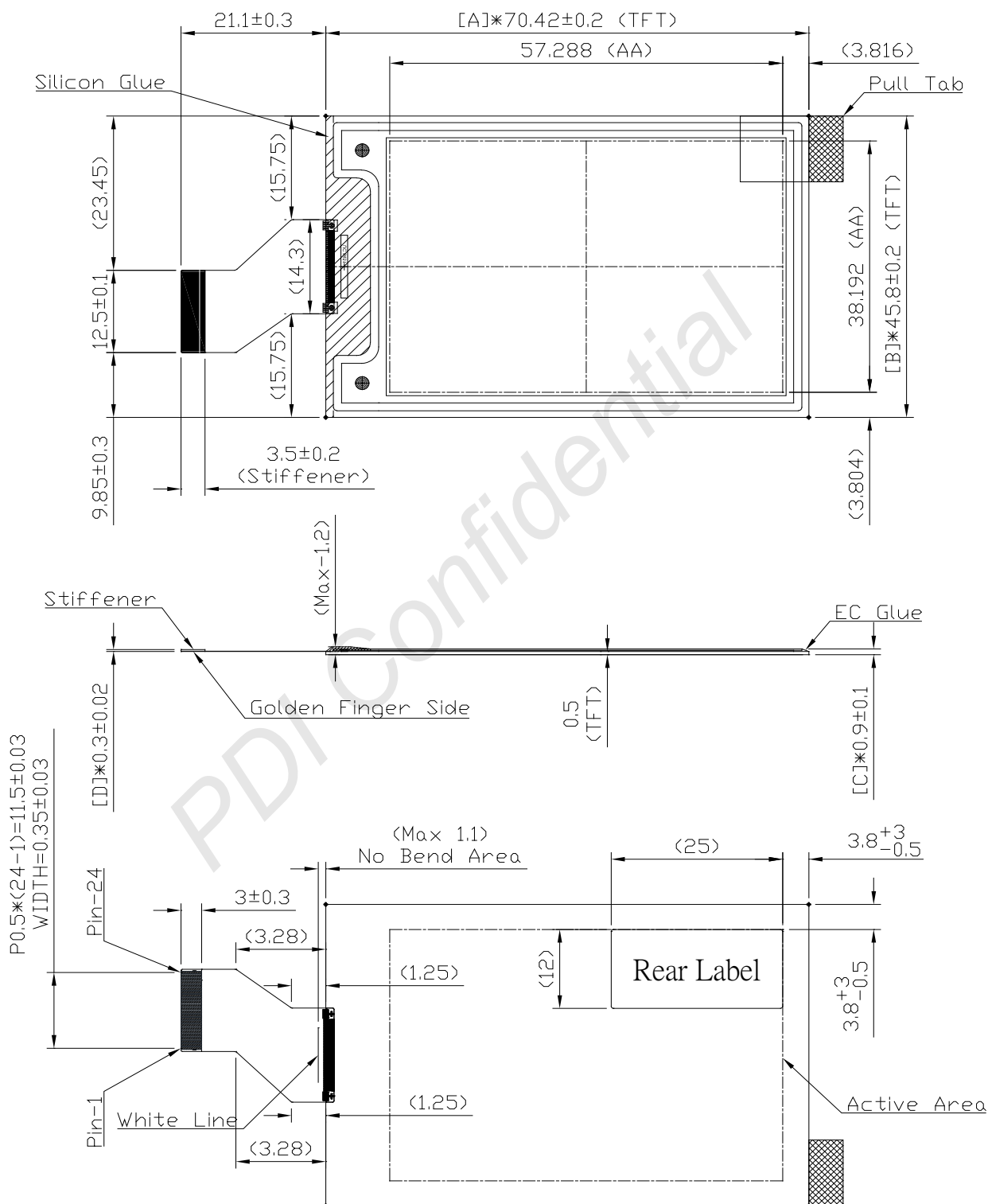
Figure 1-1 EPD Drawing
