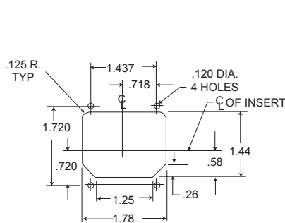
-34 Front Mount
