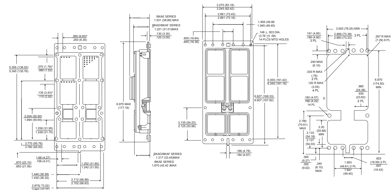
Retainer Plate
