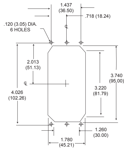
Rear Mount
