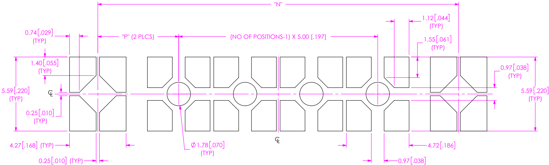
FIG 7 D STENCIL FOR GRF7-J-P-04-XX-ST-TH1-X SHOWN (DIFFERENT AS SHOWN, OTHERWISE SAME AS FIG 1)
