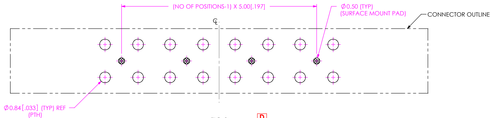
FIG 2 FOOTPRINT FOR GRF7-J-P-04-XX-ST-MT1 SHOWN (SAME AS FIG 1 EXCEPT AS NOTED)
