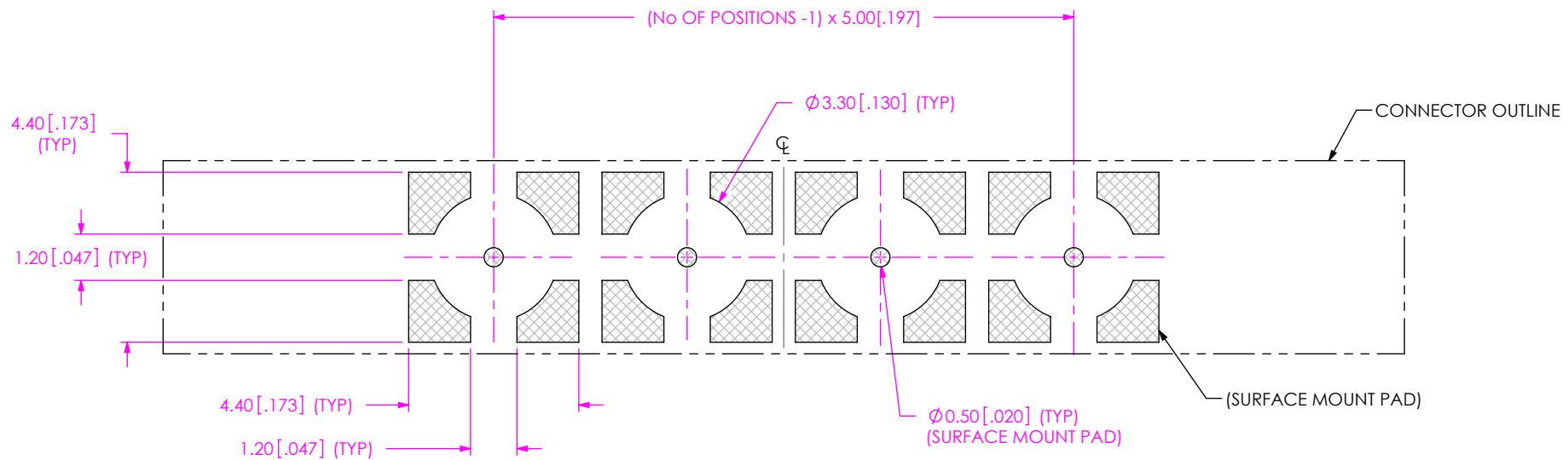
FIG 4 FOOTPRINT FOR GRF7-J-P-04-XX-ST-SM1 SHOWN D (SAME AS FIG 1 EXCEPT AS NOTED)
