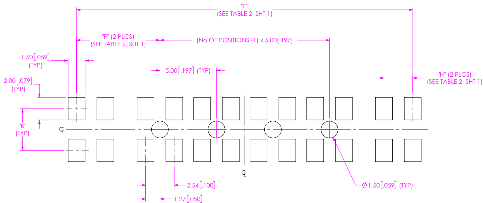
FIG 6 STENCIL FOR GRFX-J-P-04-XX-RA-TH1 WITH -E OPTION SHOWN C (DIFFERENT AS SHOWN, OTHERWISE SAME AS FIG 1)
