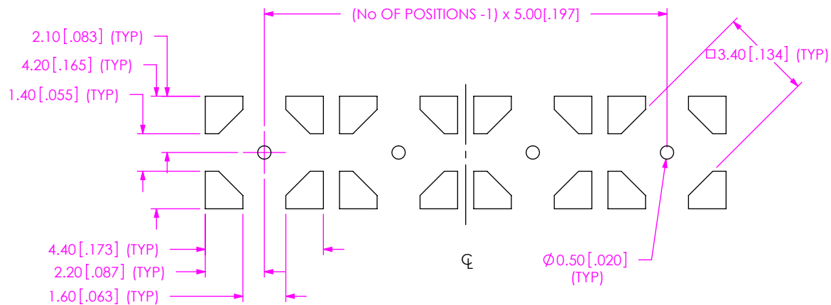
FIG 3 STENCIL FOR GRF7-J-P-04-XX-RA-MT1 (SAME AS FIG 1, EXCEPT AS NOTED) (SEE NOTE 1, SHT 4)
