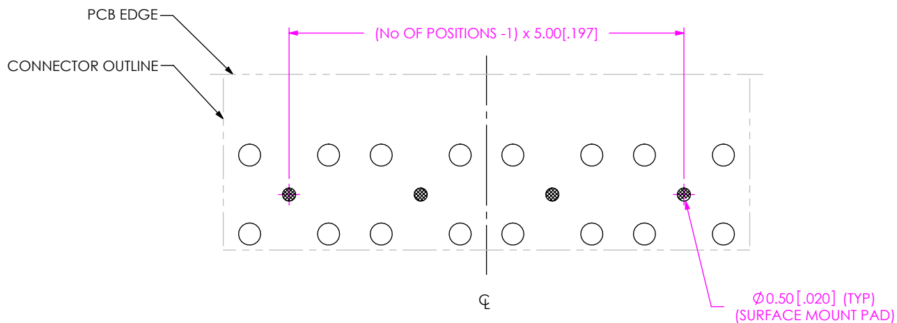
FIG 2 FOOTPRINT FOR GRF7-J-P-04-XX-RA-MT1 SHOWN C (SAME AS FIG 1, EXCEPT AS NOTED)
