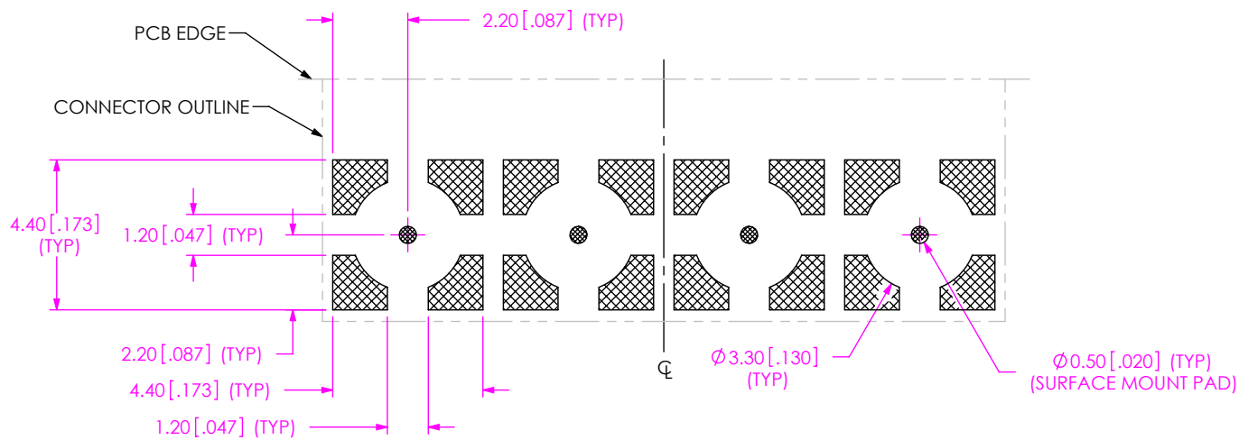
FIG 4 FOOTPRINT FOR GRF7-J-P-04-XX-RA-SM1 SHOWN C (SAME AS FIG 1, EXCEPT AS NOTED)
