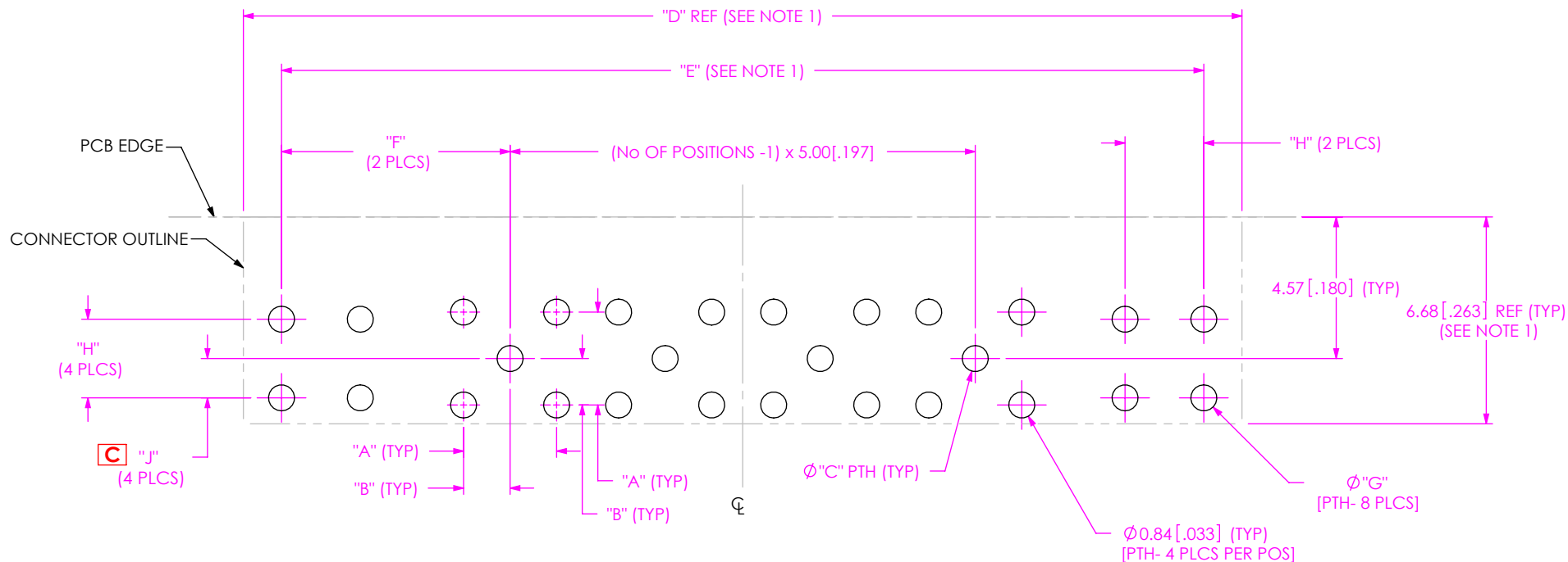
FIG 1 FOOTPRINT FOR GRFX-J-P-04-XX-RA-TH1 WITH -E OPTION SHOWN
