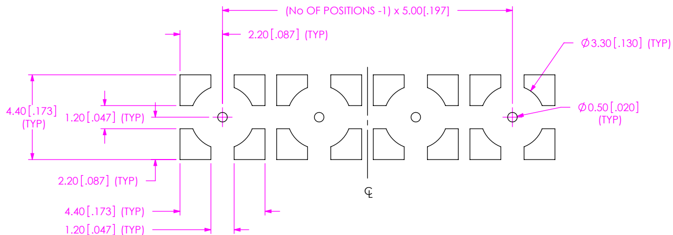
FIG 5 STENCIL FOR GRF7-J-P-04-XX-RA-SM1 SHOWN C (SAME AS FIG 1, EXCEPT AS NOTED) (SEE NOTE 1, SHT 6)
