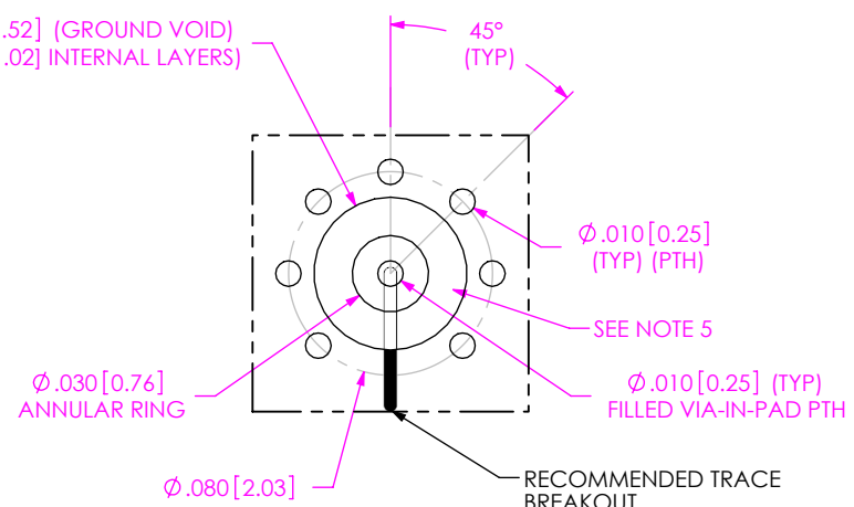
DETAIL 'A' SCALE 12:1 (TYPICAL ON ALL POSITIONS)
