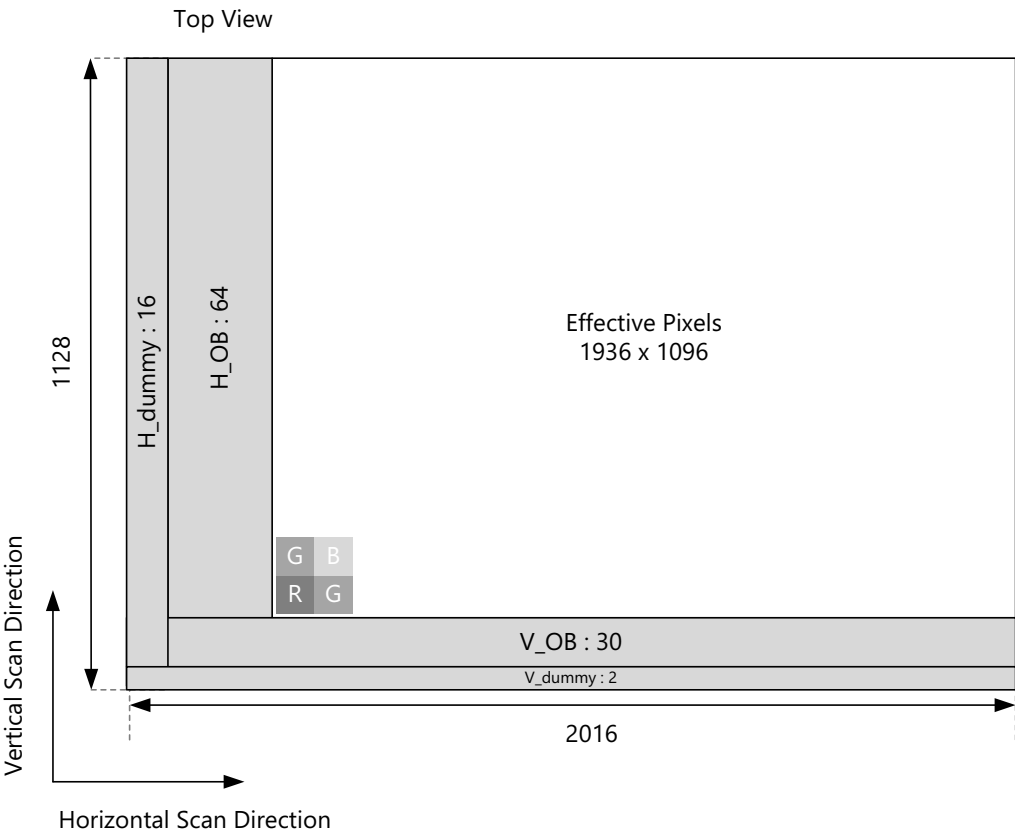
Figure 3-1. Pixel Data Format (Physical Arrangement)
