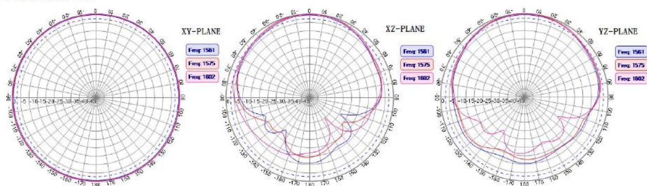
GNSS Antenna
