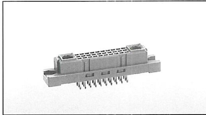
Female connector contact spacing .100" and .200" for signal contacts Solder Technology and wire wrap
