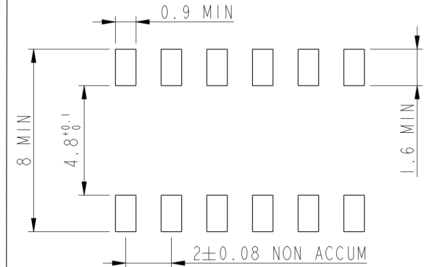
RECOMMENDED PAD LAYOUT
