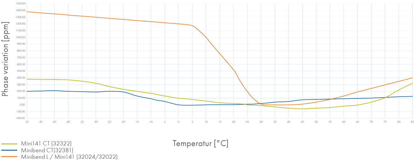
Phase variation vs. temperature
