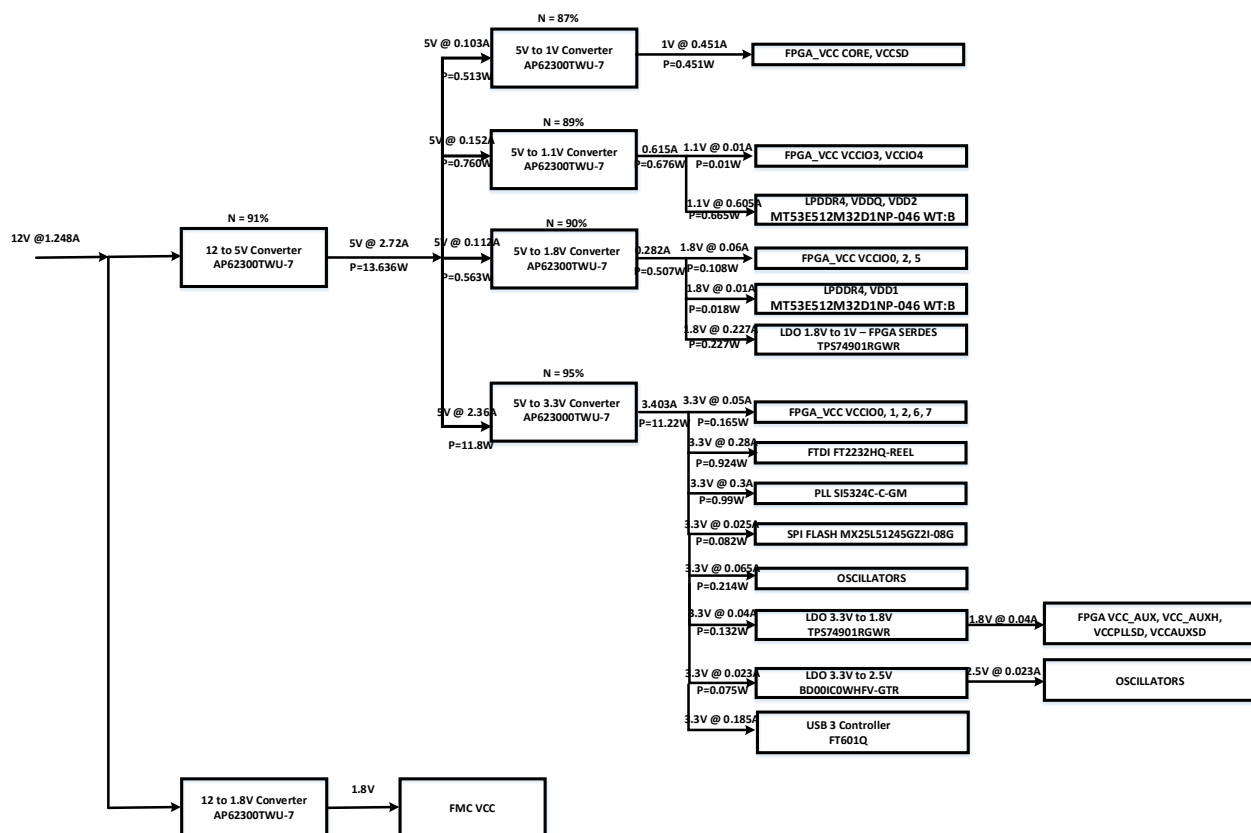
Figure 5.1. Power Scheme
