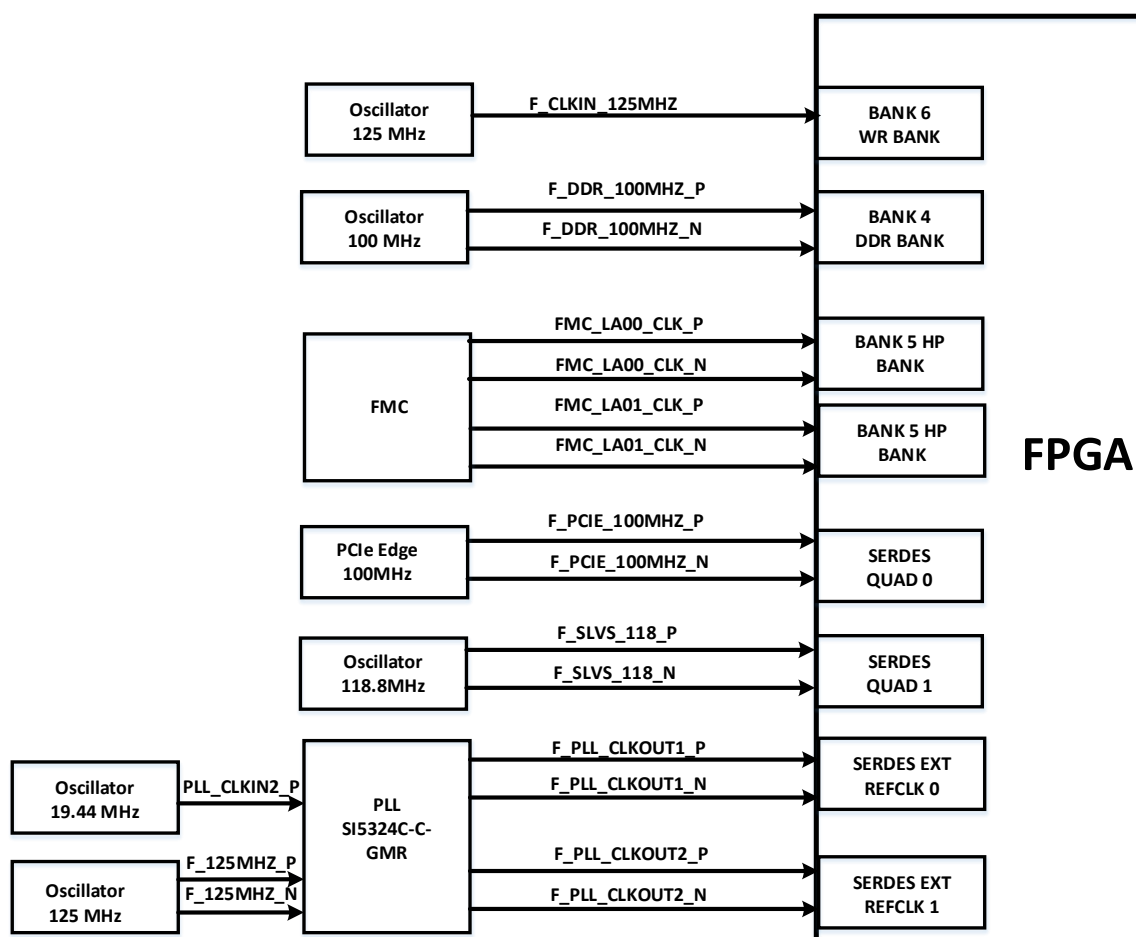
Figure 4.1. Clock Scheme
