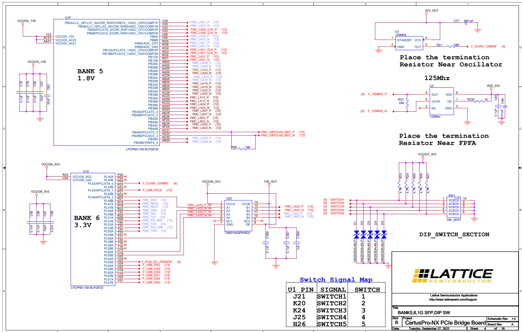
Figure A. 4. BANK5,6,1G SFP,DIP SW
