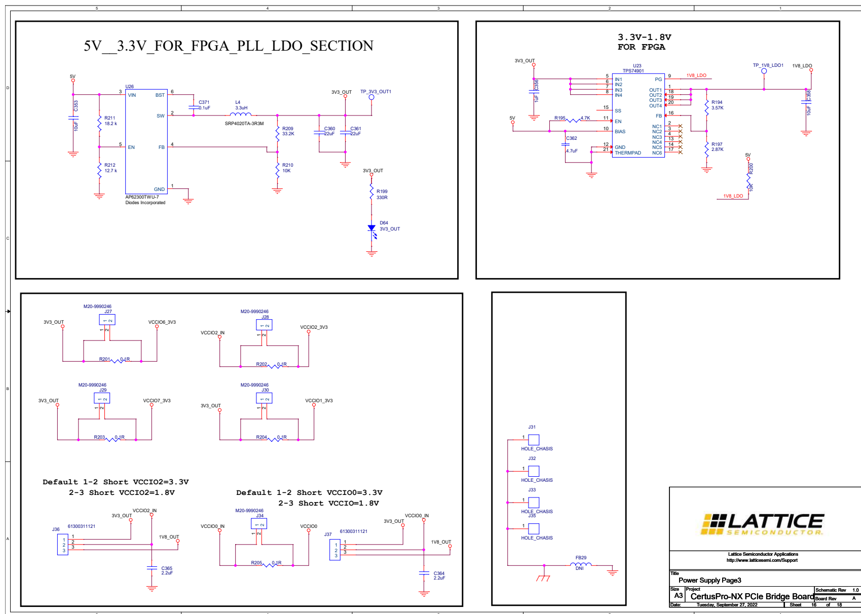
Figure A. 16. Power Supply Page3
