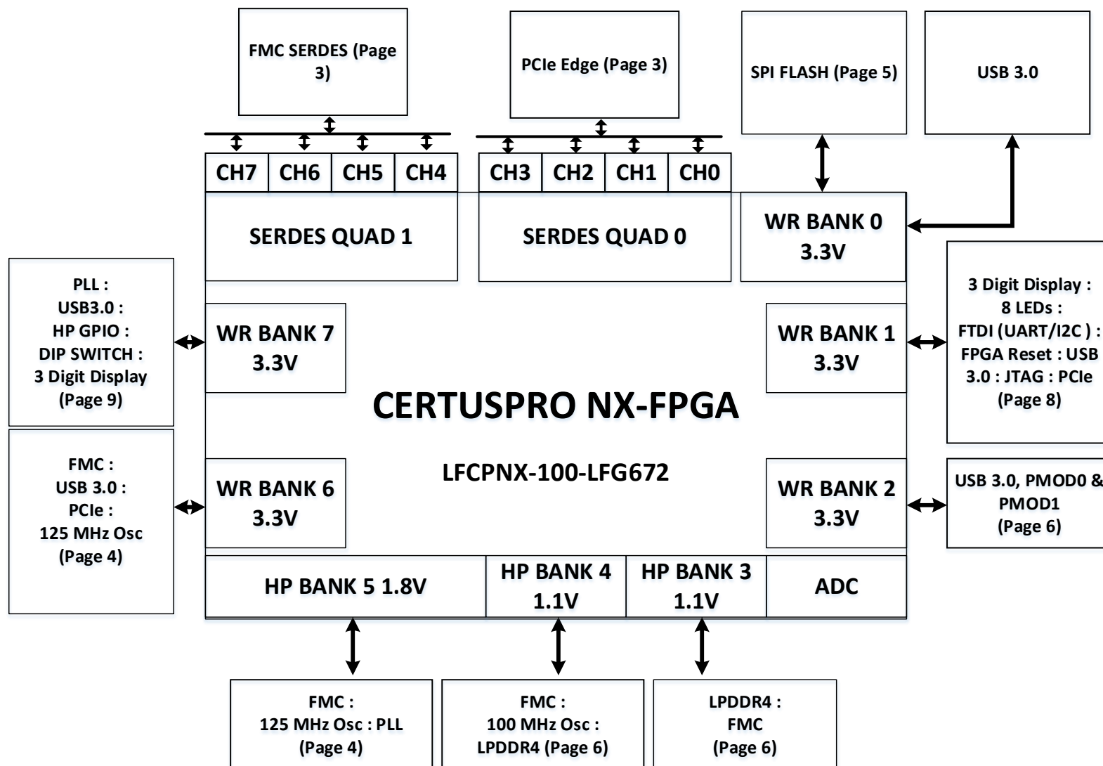
Figure A. 2. Block Diagram
