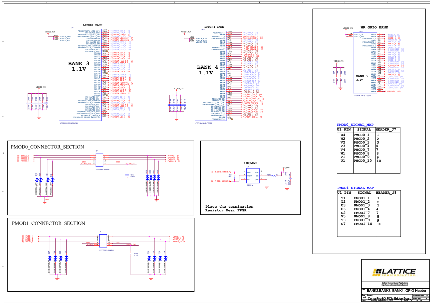
Figure A. 6. BANK2, BANK3, BANK4, GPIO Header
