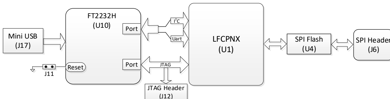
Figure 3.1. Configuration Architecture
