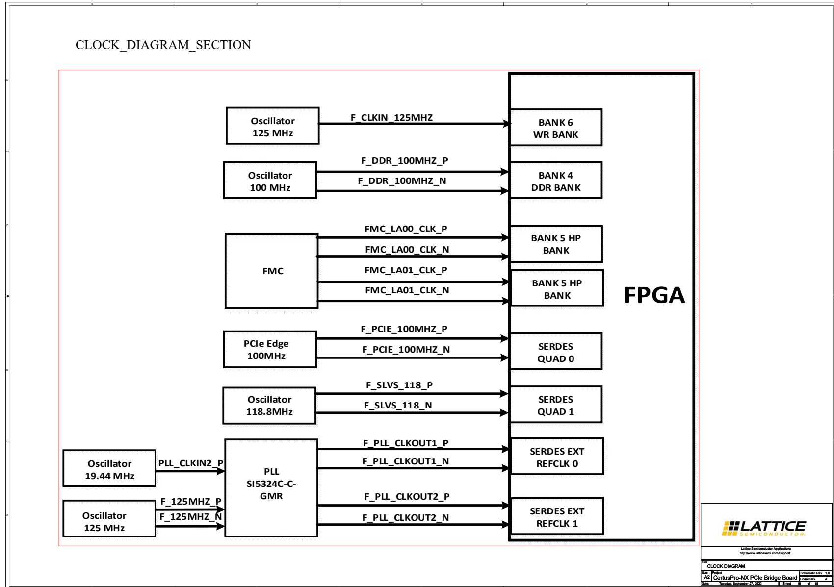
Figure A. 18. CLOCK DIAGRAM
