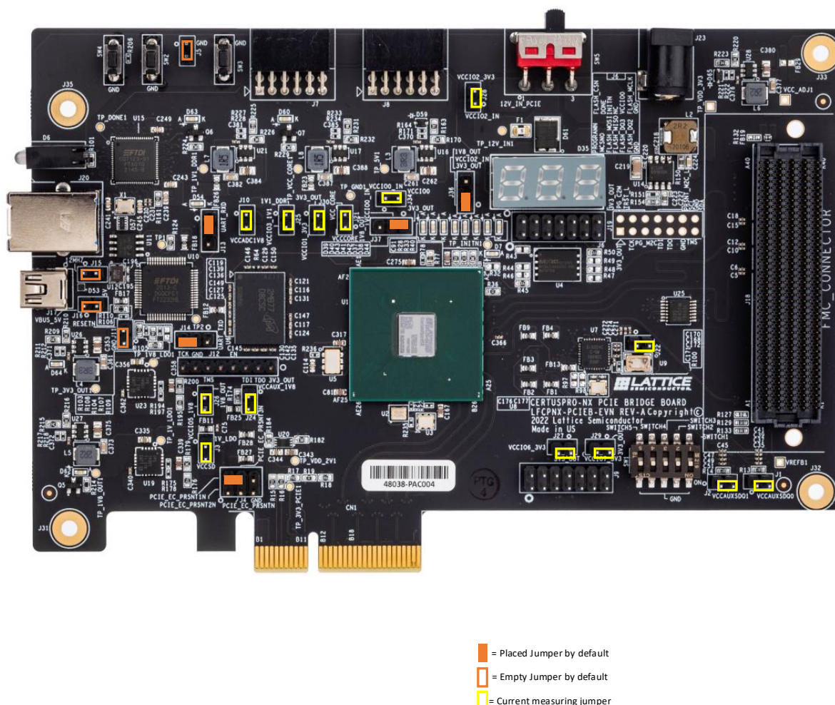
Figure 2.1. Top View of CertusPro-NX PCIe Bridge Board – Jumper Selection
