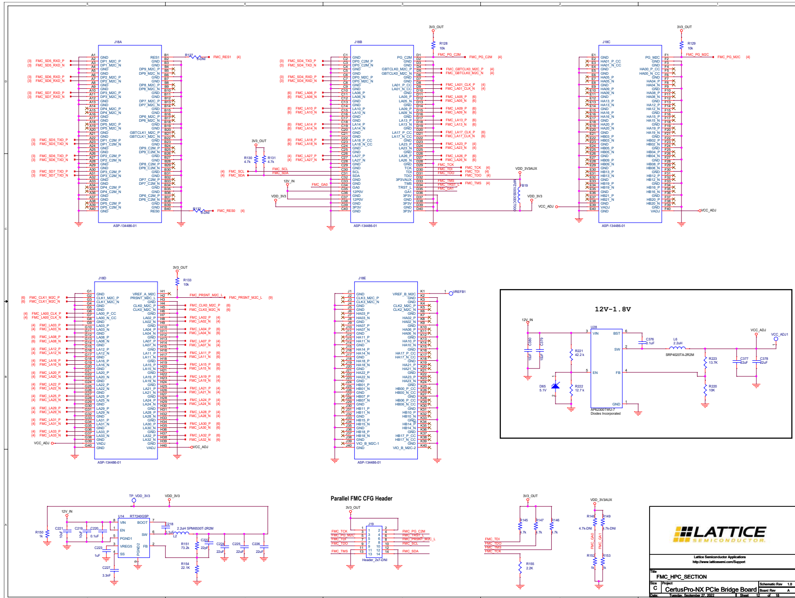
Figure A. 12. FMC_HPC_SECTION
