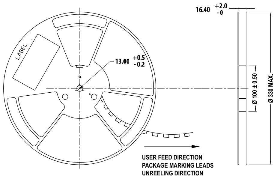
Figure 14: Reel Dimensions
