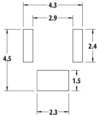
Figure 12: Recommended Soldering Pad Pattern
