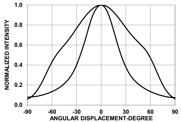
Figure 10: Radiation Pattern
