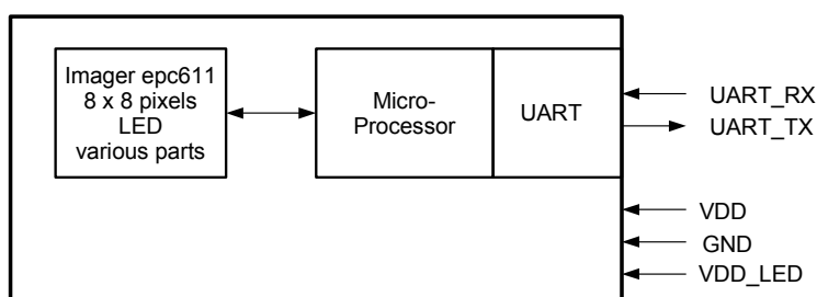
Figure 3: Block diagram
