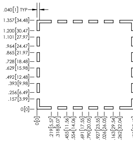
PCB FOOTPRINT
