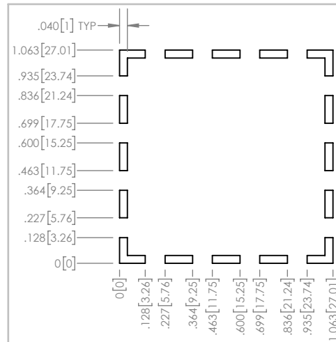
PCB FOOTPRINT
