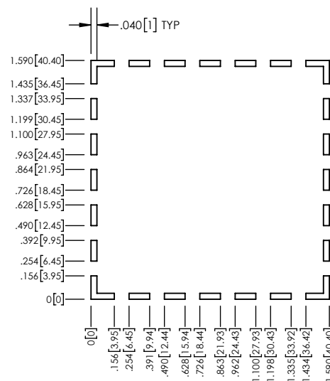
PCB FOOTPRINT
