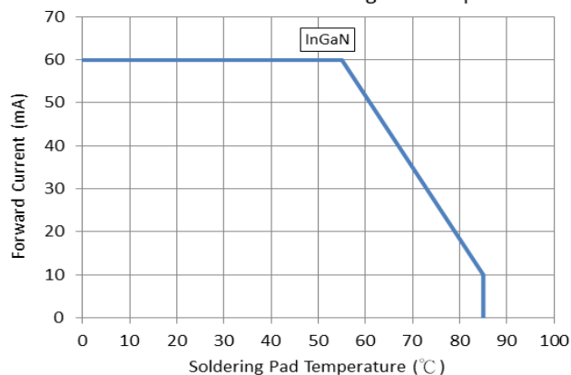
Forward Current vs. Soldering Pad Temperature
