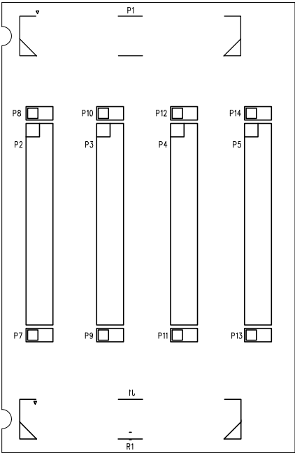
Figure 2-1. Connector Locations
