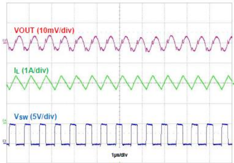
Figure 8. Output Voltage Ripple, IO UT = 2A
