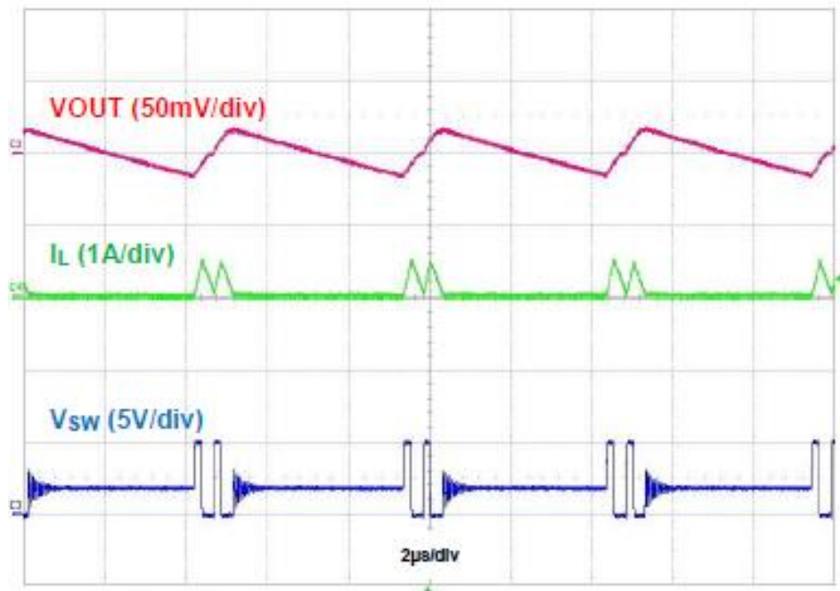
Figure 7. Output Voltage Ripple, IO UT = 50mA
