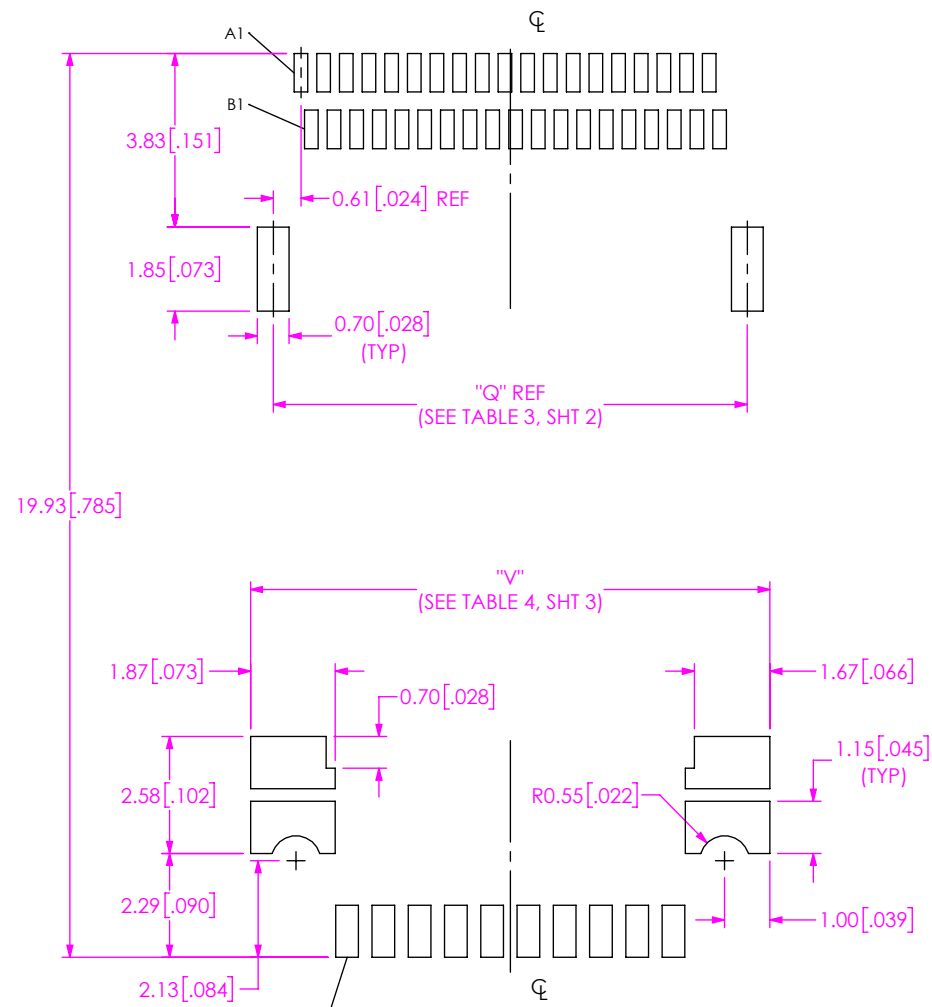
FIG 6 UEC5-019-1-X-D-RA-2-X STENCIL SHOWN UCC8-010-X-X-S-2-A STENCIL SHOWN (DIFFERENT AS SHOWN, OTHERWISE SAME AS FIG 5) (AVAILABLE FOR EXISTING CUSTOMERS ONLY)
