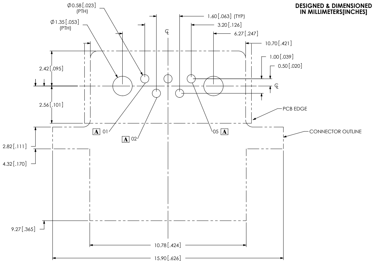
FIG. 1 SPM-05-S-B-RA-PF-XX SHOWN
